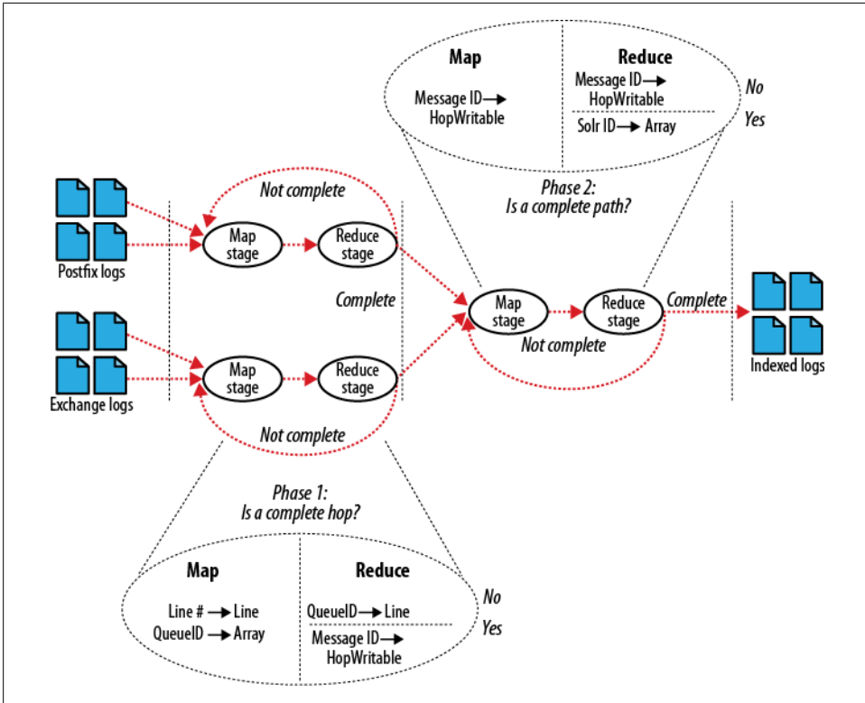
Figure 16-9. MapReduce chain
