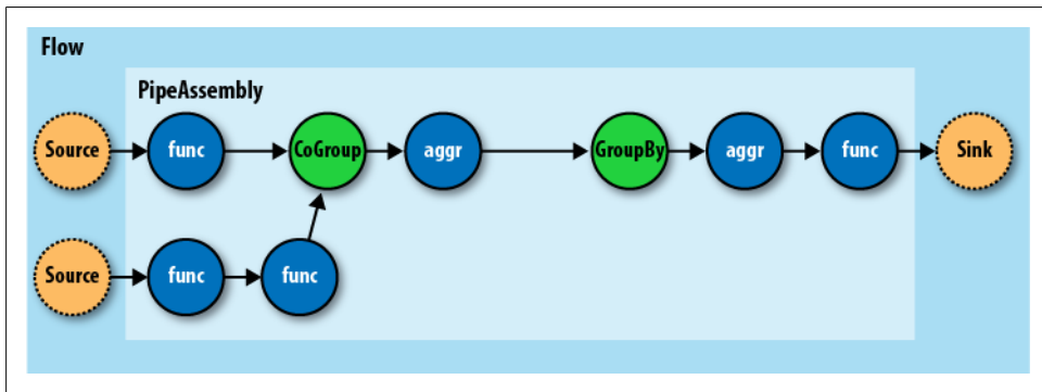
Figure 16-17. A Flow
