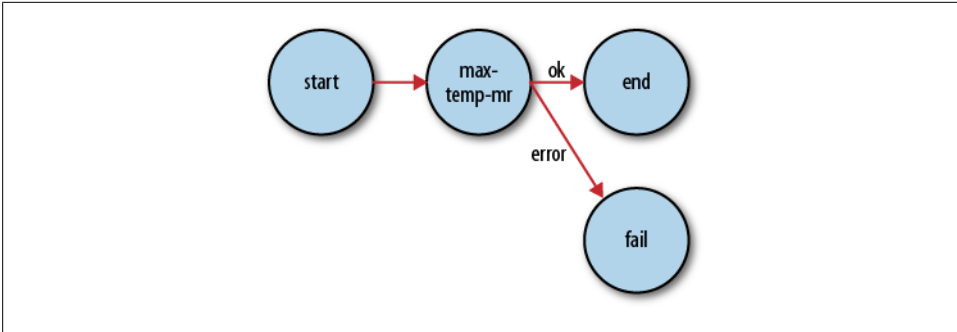
Figure 5-5. Transition diagram of an Oozie workflow
