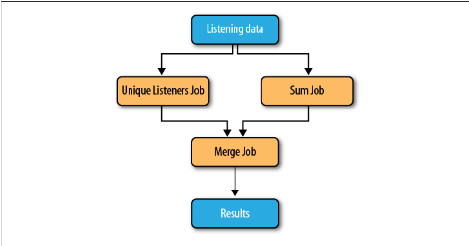
Figure 16-2. TrackStats jobs
