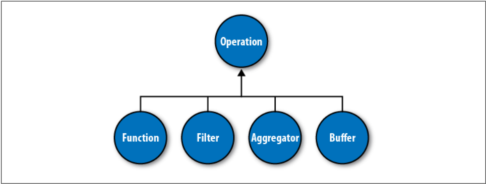
Figure 16-15. Operation types
