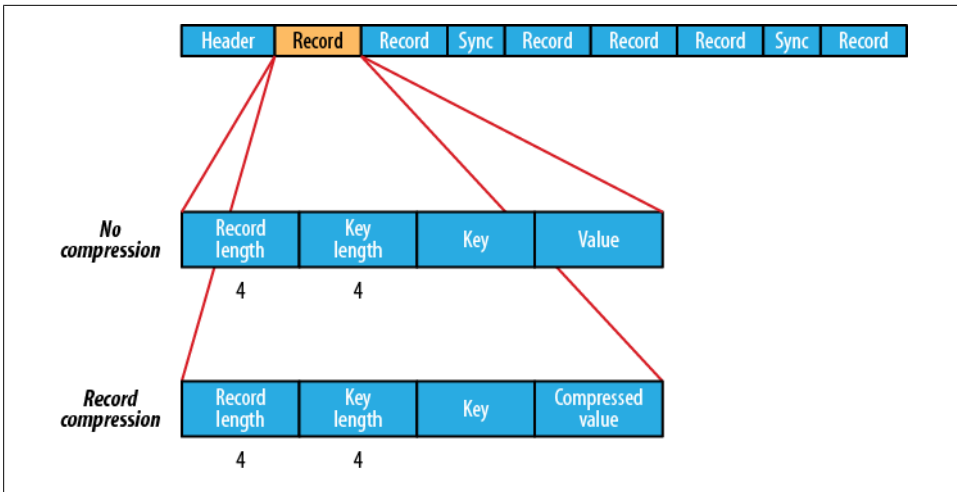
Figure 4-2. The internal structure of a sequence file with no compression and with record compression
