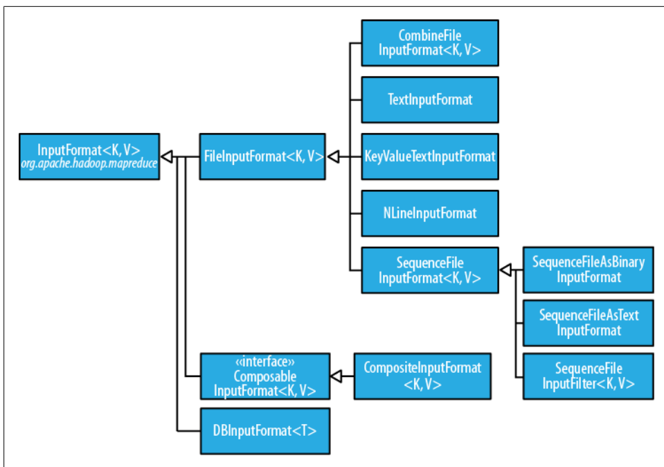
Figure 7-2. InputFormat class hierarchy
