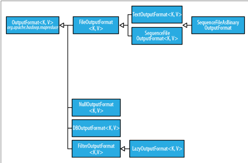
Figure 7-4. OutputFormat class hierarchy
