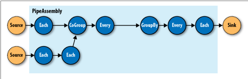
Figure 16-14. A simple PipeAssembly
