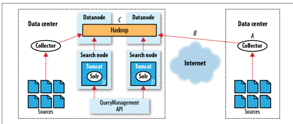
Figure 16-8. Hadoop data flow at Rackspace
