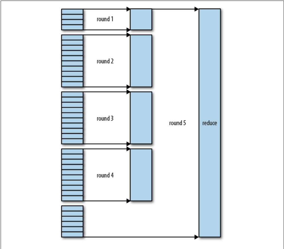
Figure 6-7. Efficiently merging 40 file segments with a merge factor of 10
