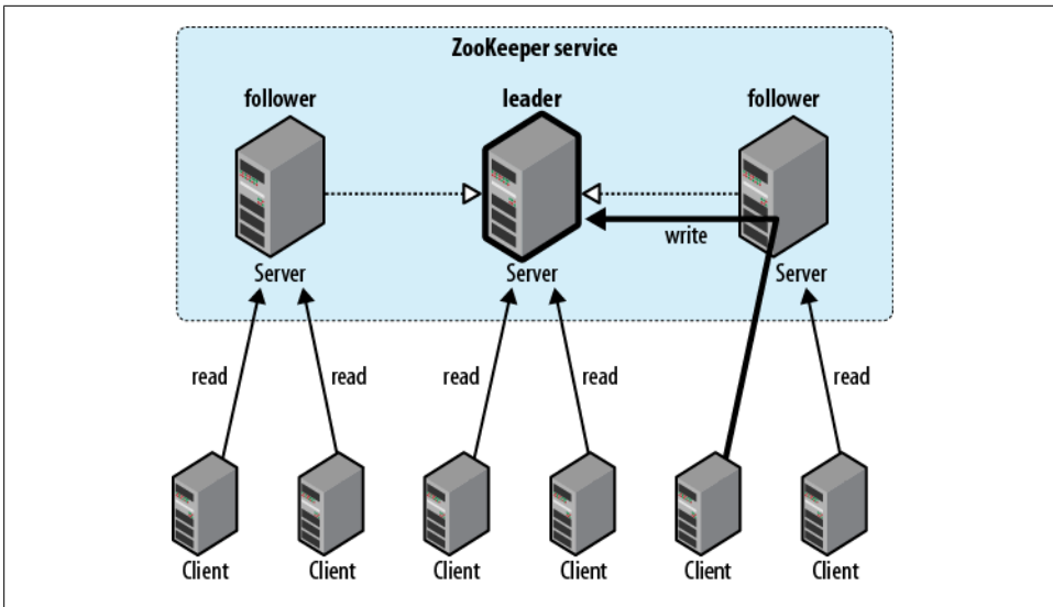
Figure 14-2. Reads are satisfied by followers, whereas writes are committed by the leader
