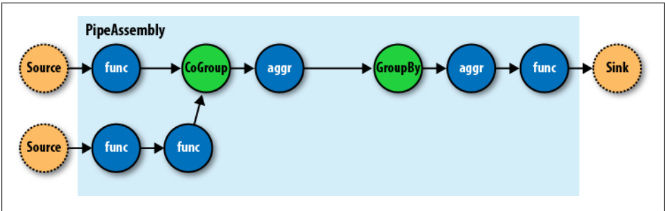
Figure 16-16. An assembly of operations
