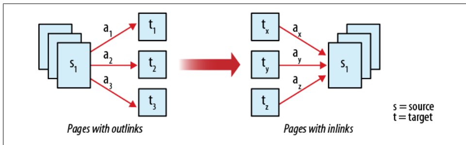
Figure 16-6. Link inversion
