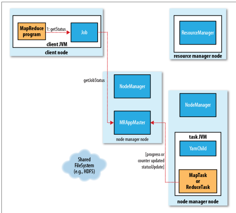
Figure 6-5. How status updates are propagated through the MapReduce 2 system
