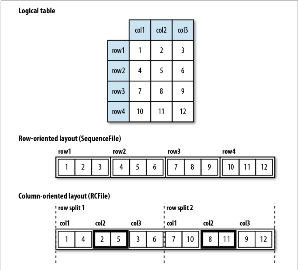
Figure 12-3. Row-oriented versus column-oriented storage
