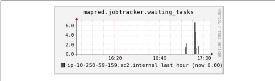
Figure 10-2. Ganglia plot of the number of tasks in the jobtracker queue
