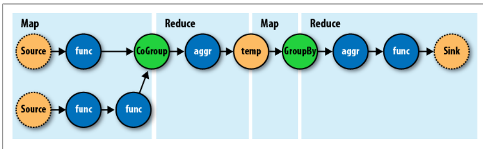
Figure 16-18. How a Flow translates to chained MapReduce jobs
